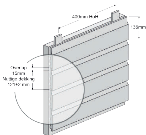
18 x 136 Cove
