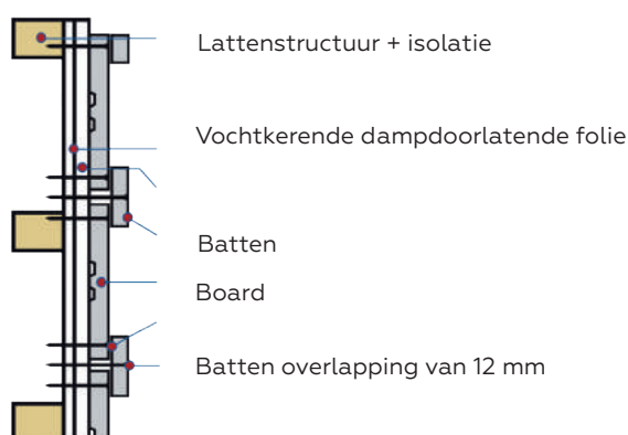
CLASSIC BOARDS & BATTENS 18 x 180 mm 18 x 68 mm
