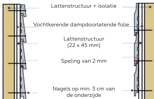
CLASSIC BEVEL 22 x 136 mm
