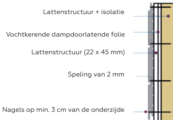
NEO EVOLUTION 18 x 136 mm
